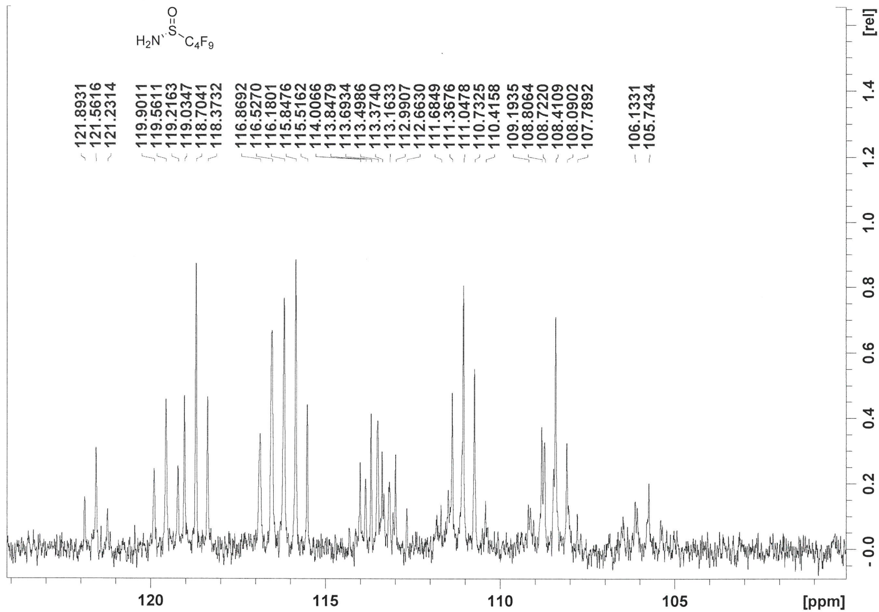
13 C NMR (100 MHz, DMSO-d 6 ) of sulfinamide (expanded)
